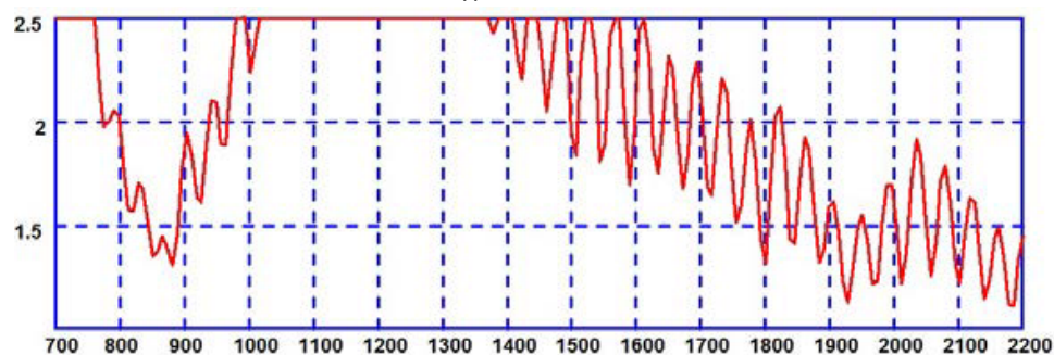
Typical VSWR
